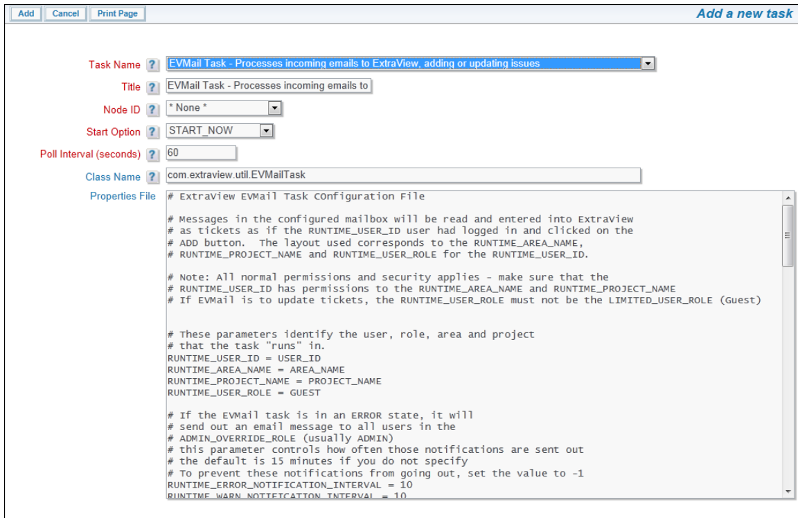
EVMail configuration screen
