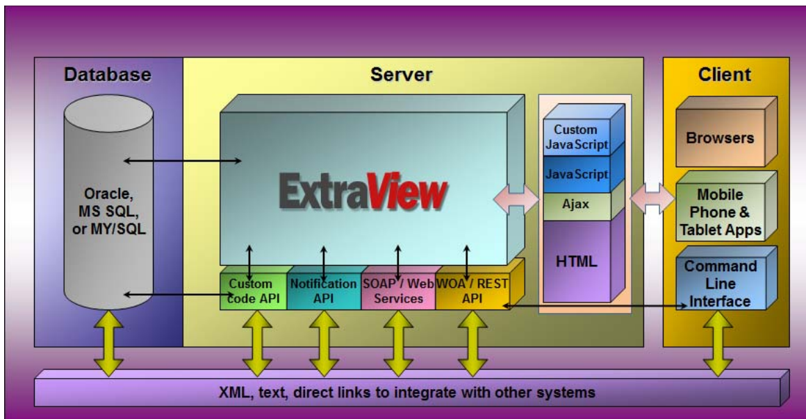
The ExtraView architecture
